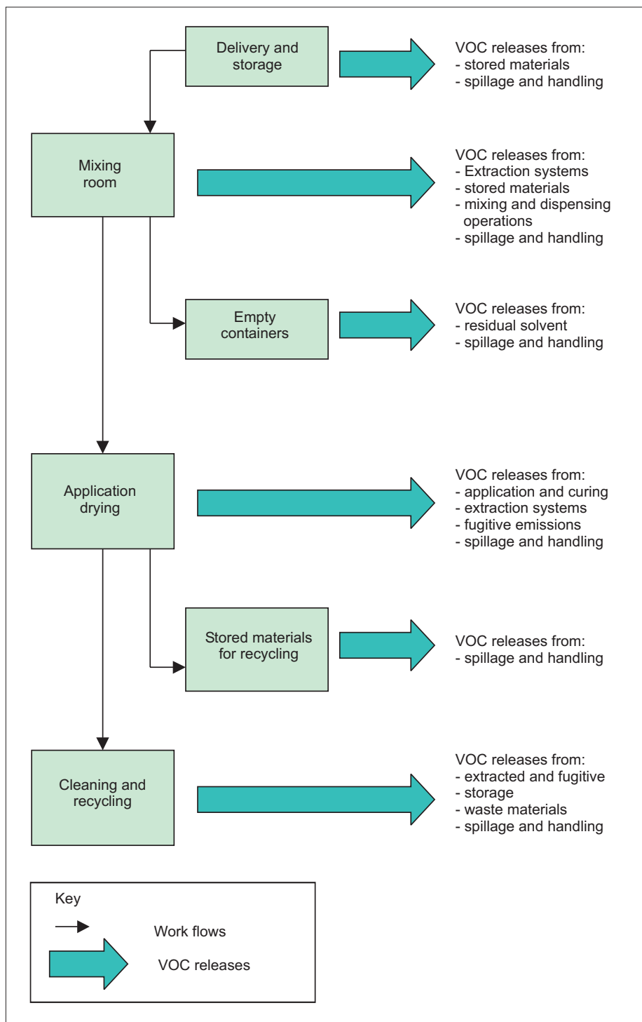
Figure 3.1: Potential VOC releases from a typical leather finishing operation
